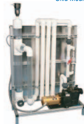
Back of PZ2-24 on Skid Mount
