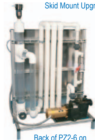
Back of PZ2-6 on Optional Skid Mount Upgrade
